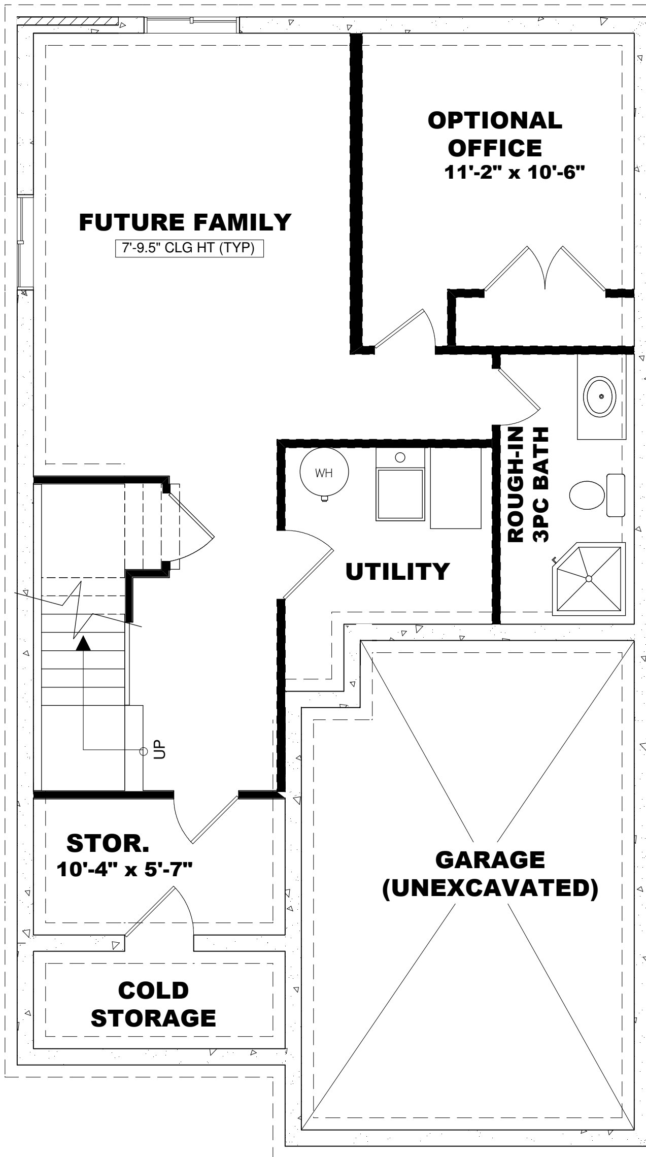
LOWER FLOOR PLAN
