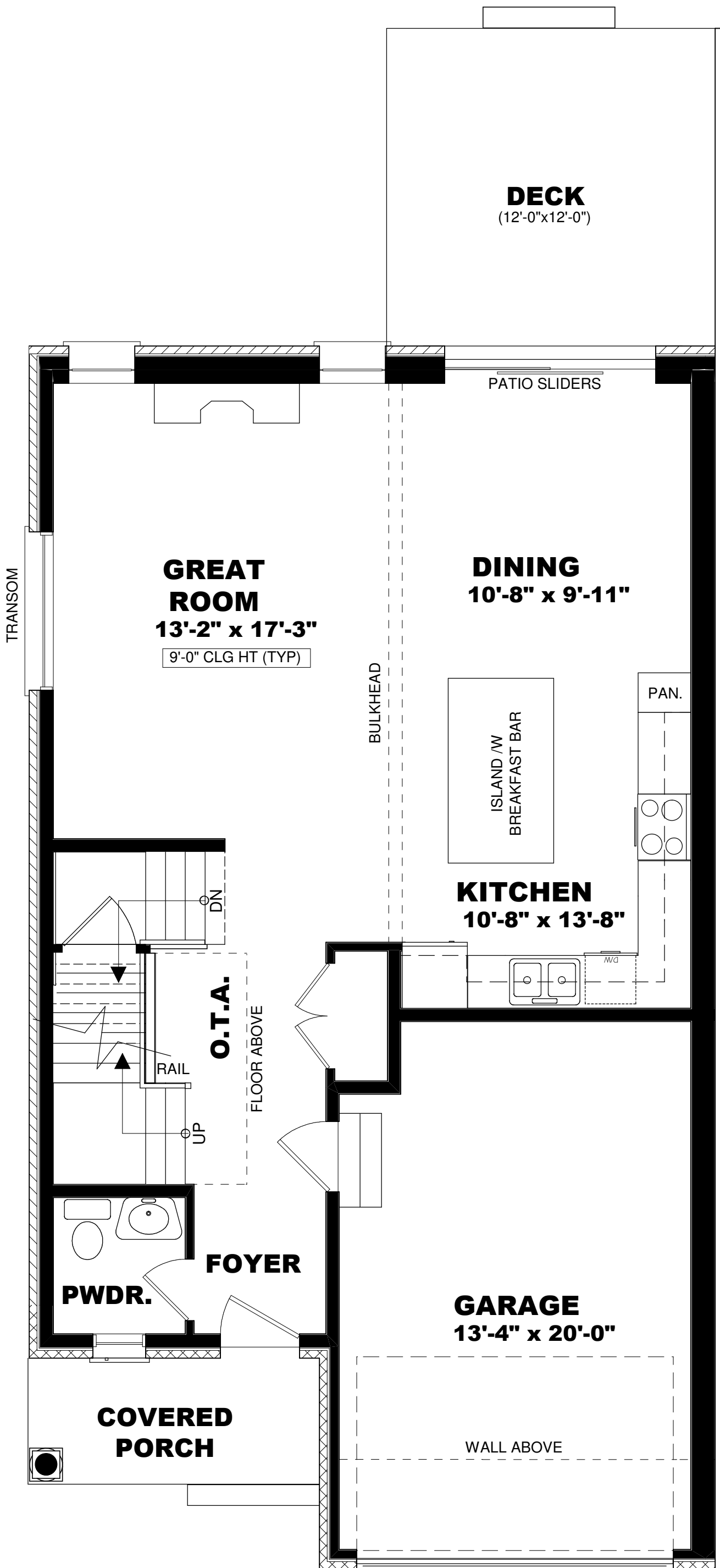
MAIN FLOOR PLAN - 821 SQ. FT TOTAL = 1793 SQ.FT (1893 SQ.FT /W O.T.B)
